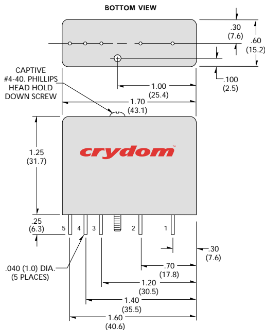
All dimensions are in inches (millimeters)
